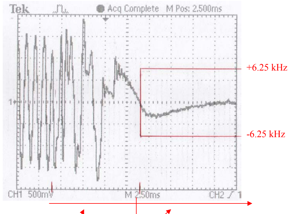
Fig. 7 Start of Transmission t_1 = 10 \text{ ms} (Unlimited deviation) t_2 = 25 \text{ ms} ( \pm 6.25 \text{ kHz} deviation or \pm 1.56 \text{ div.} )
