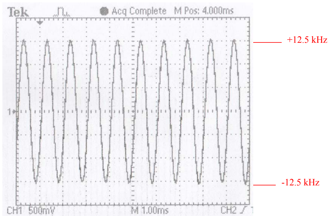
Fig. 6 \pm 12.5 kHz modulated test signal 25 kHz/6.2 div. = 4 kHz/div.
