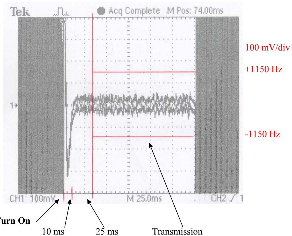
Fig. 10 Complete Transmission
