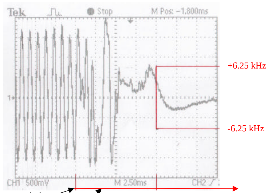
Fig. 4 Start of Transmission
