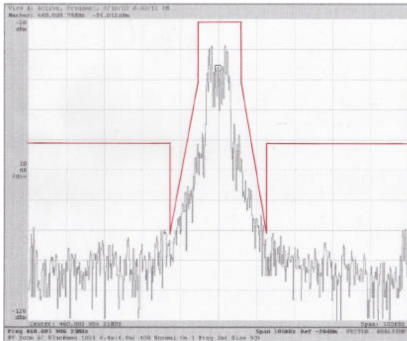
Fig. 1b Hexagram Model 8877 Electric Meter Unit Modulated Emissions Mask
