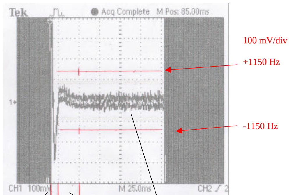
Fig. 7 Complete Transmission
