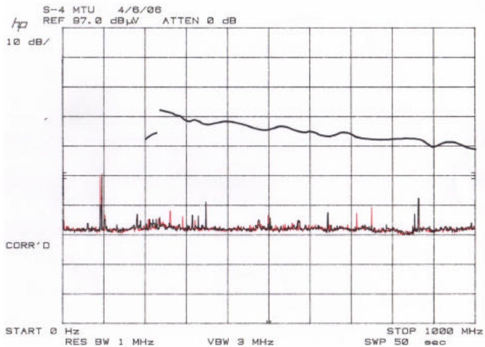
Transceiver Only
