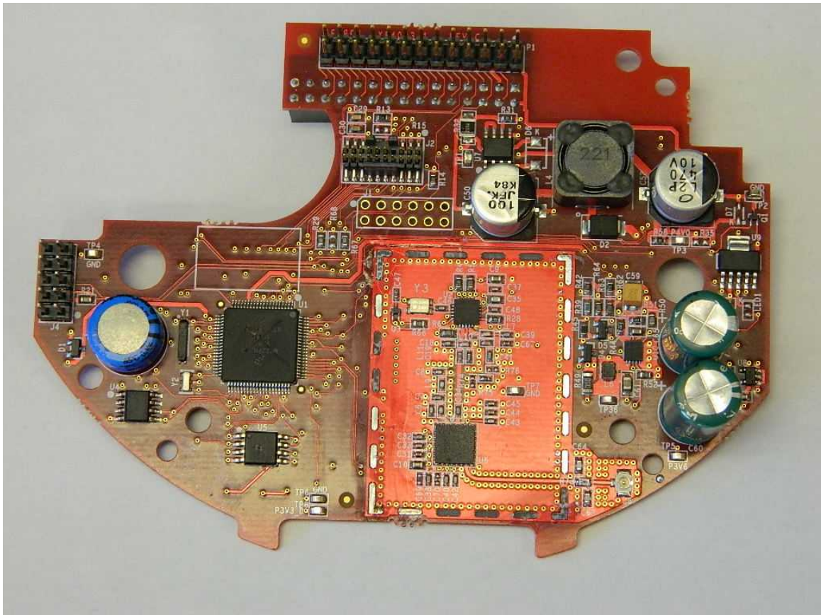
Photograph of Transmitter Board: Foil Side
