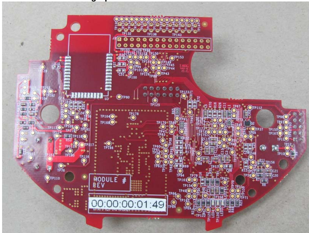
Photograph of Transmitter Board: Foil Side
