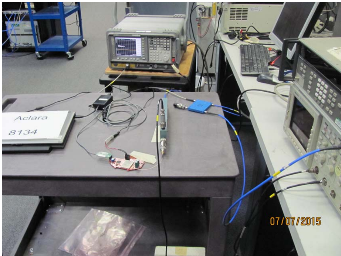
Figure 2. Photograph of Transient Frequency Behavior Test Setup
