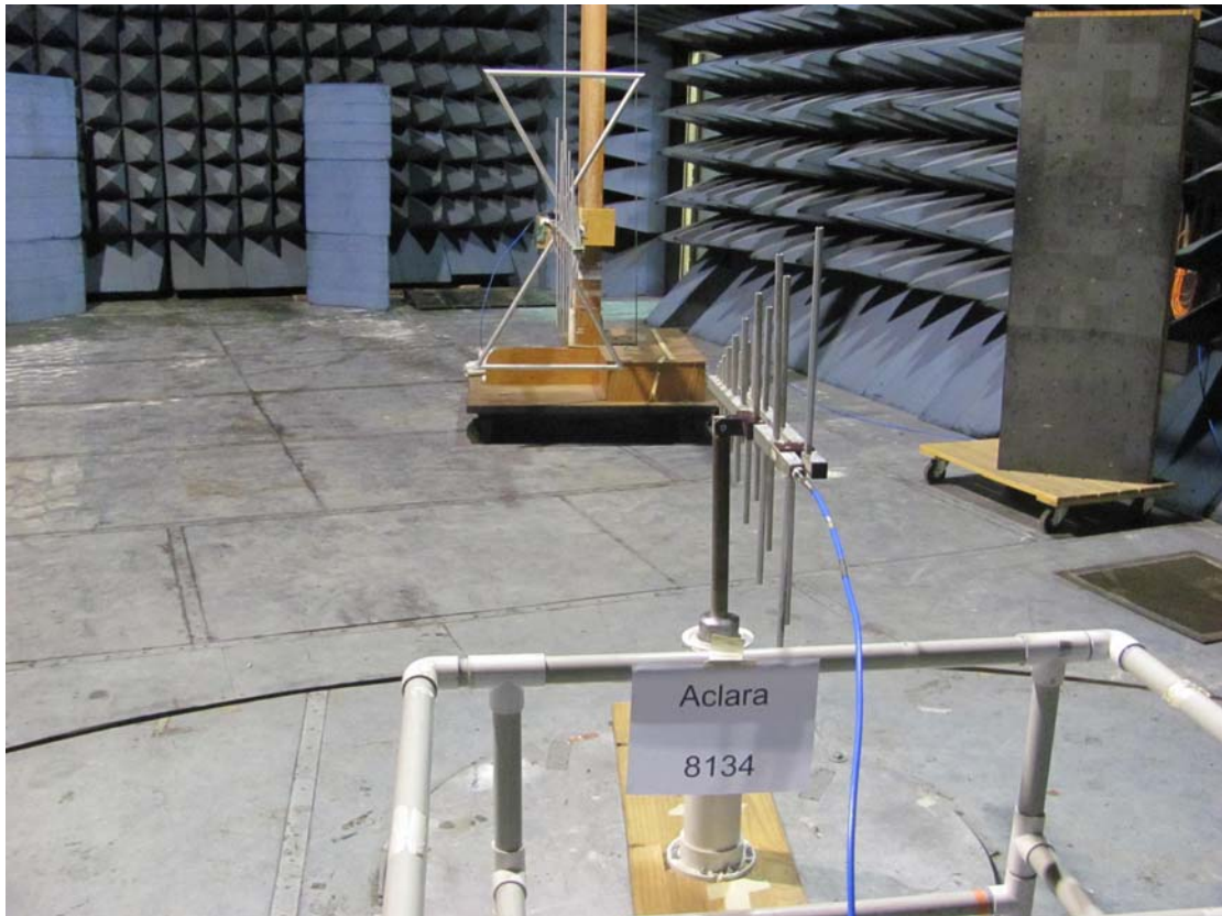
Figure 1. Photographs of Substitution Antenna Setup
