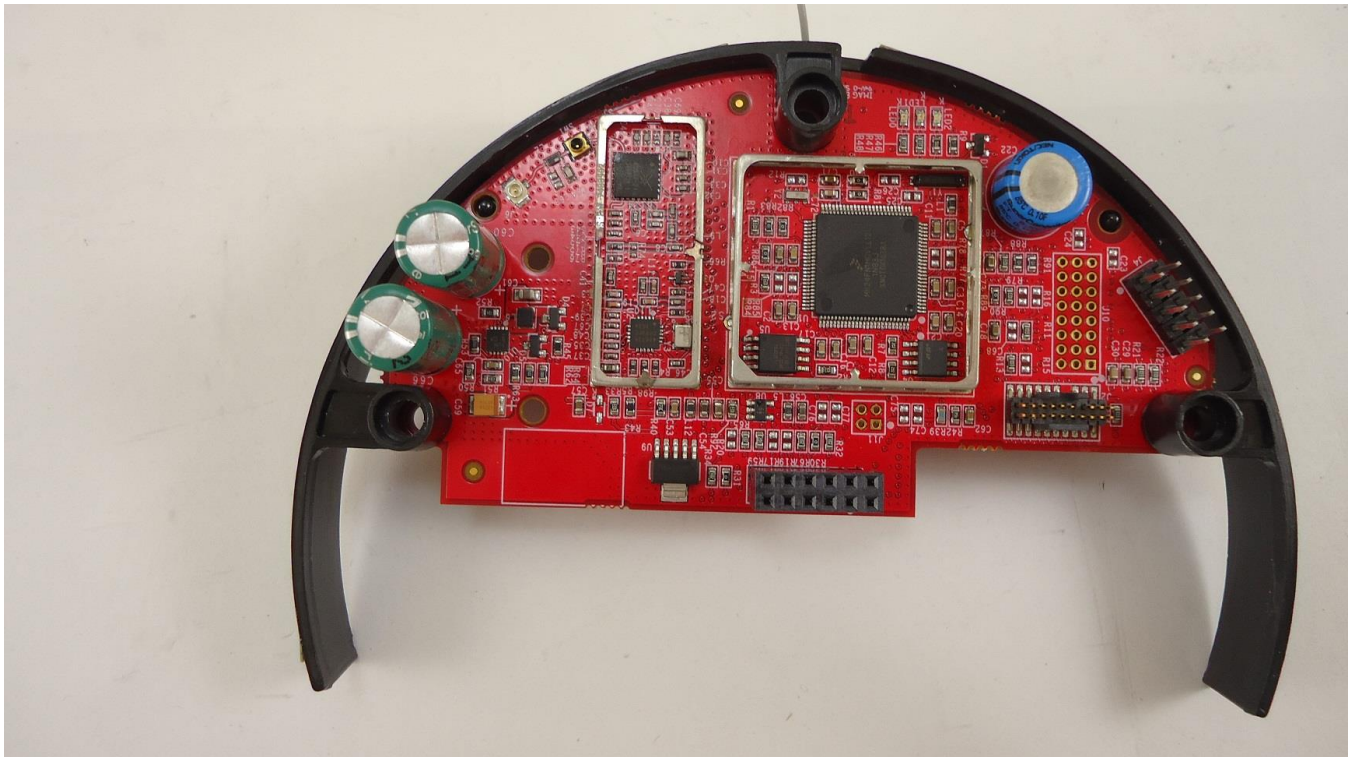
RF Board: no shields
