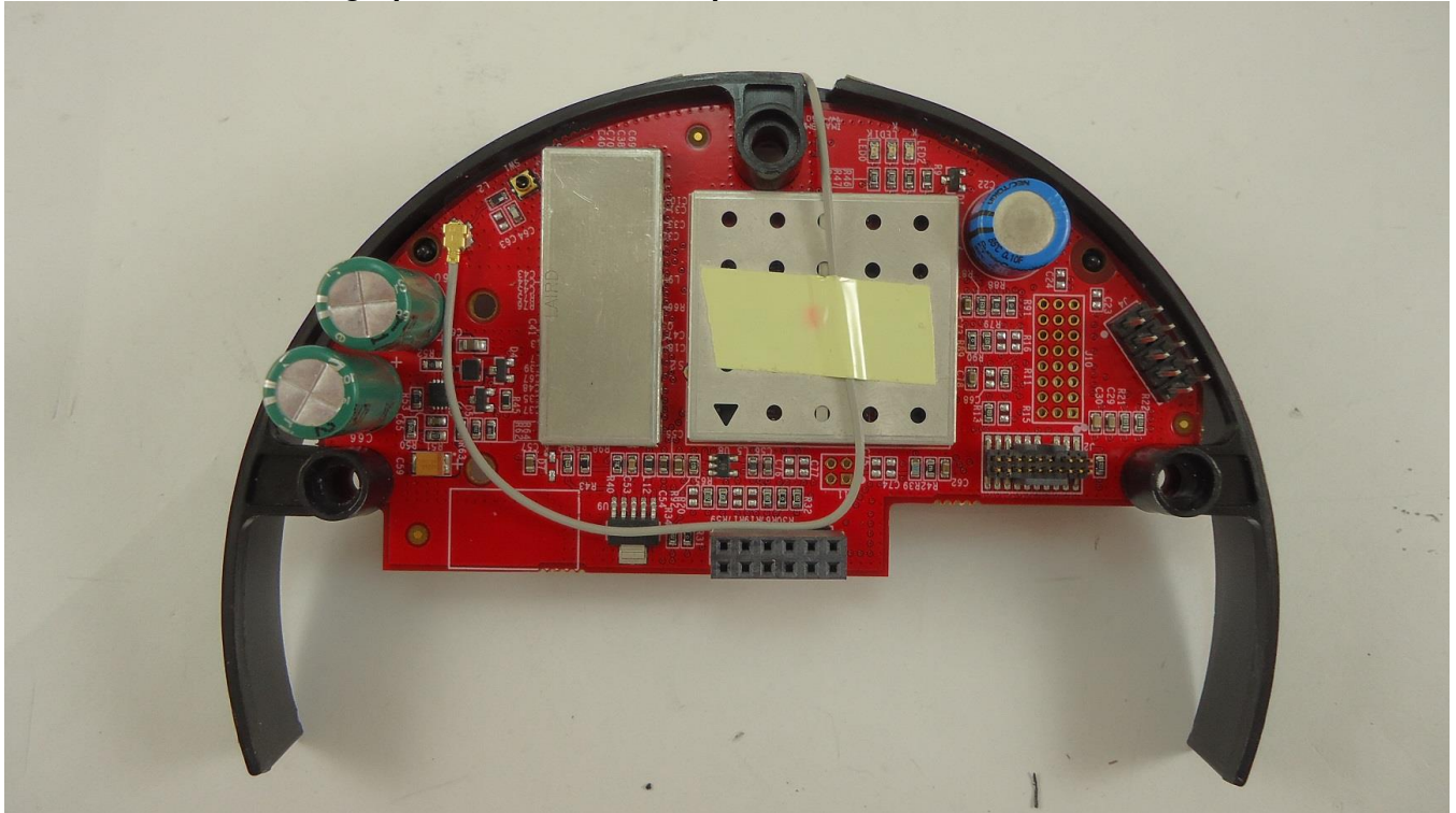
Photograph of RF Board: Component side with shield installed
