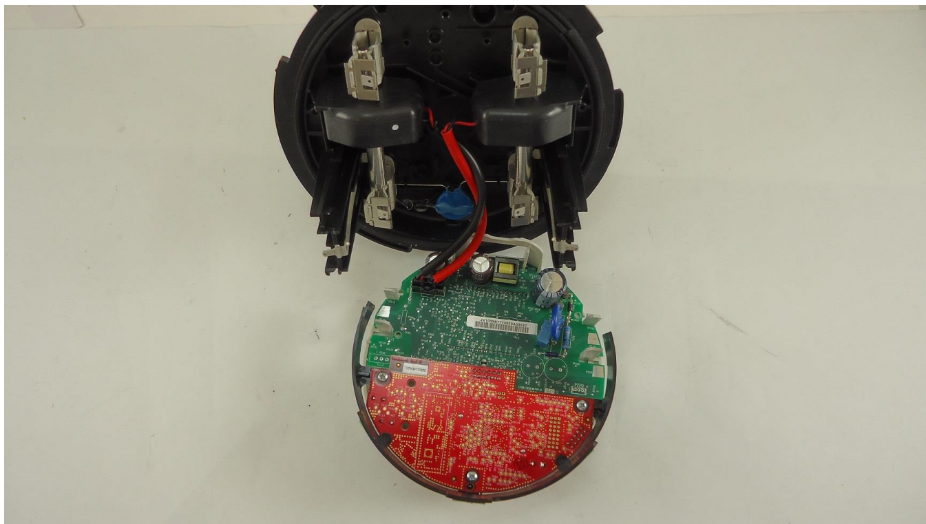
Photograph of meter assembly: cover removed
