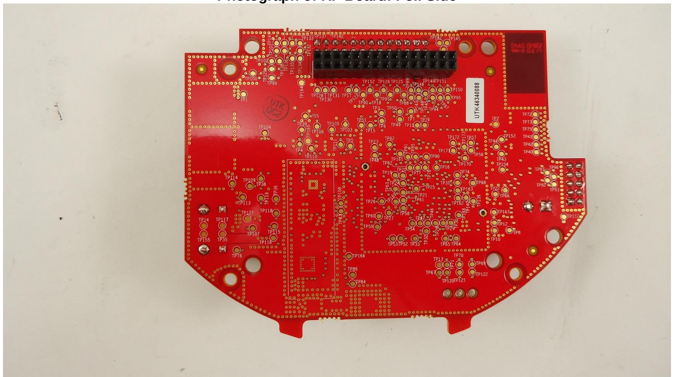
Photograph of RF Board: Foil Side
