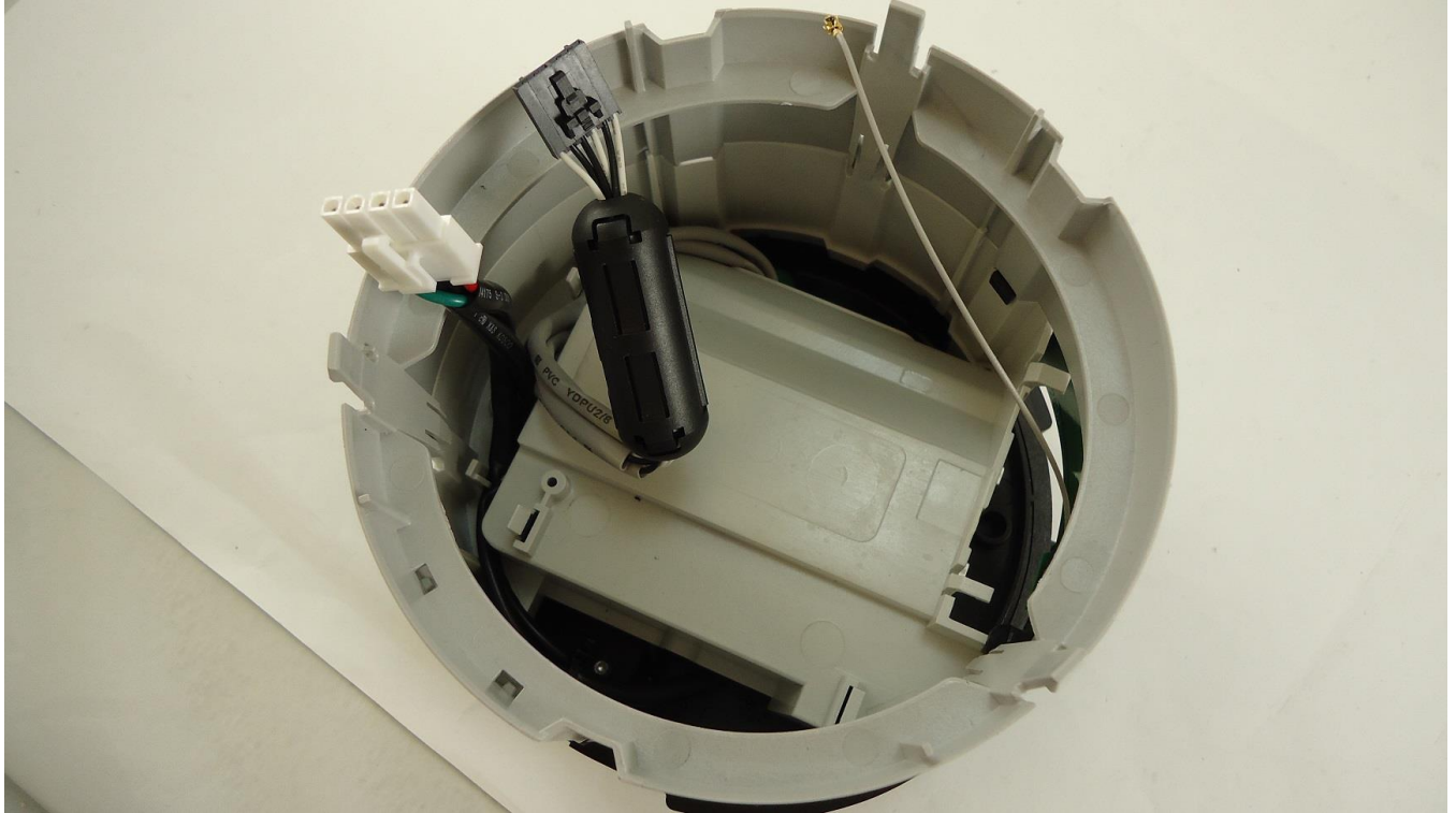
Meter base with extender and antenna carrier Inside View
