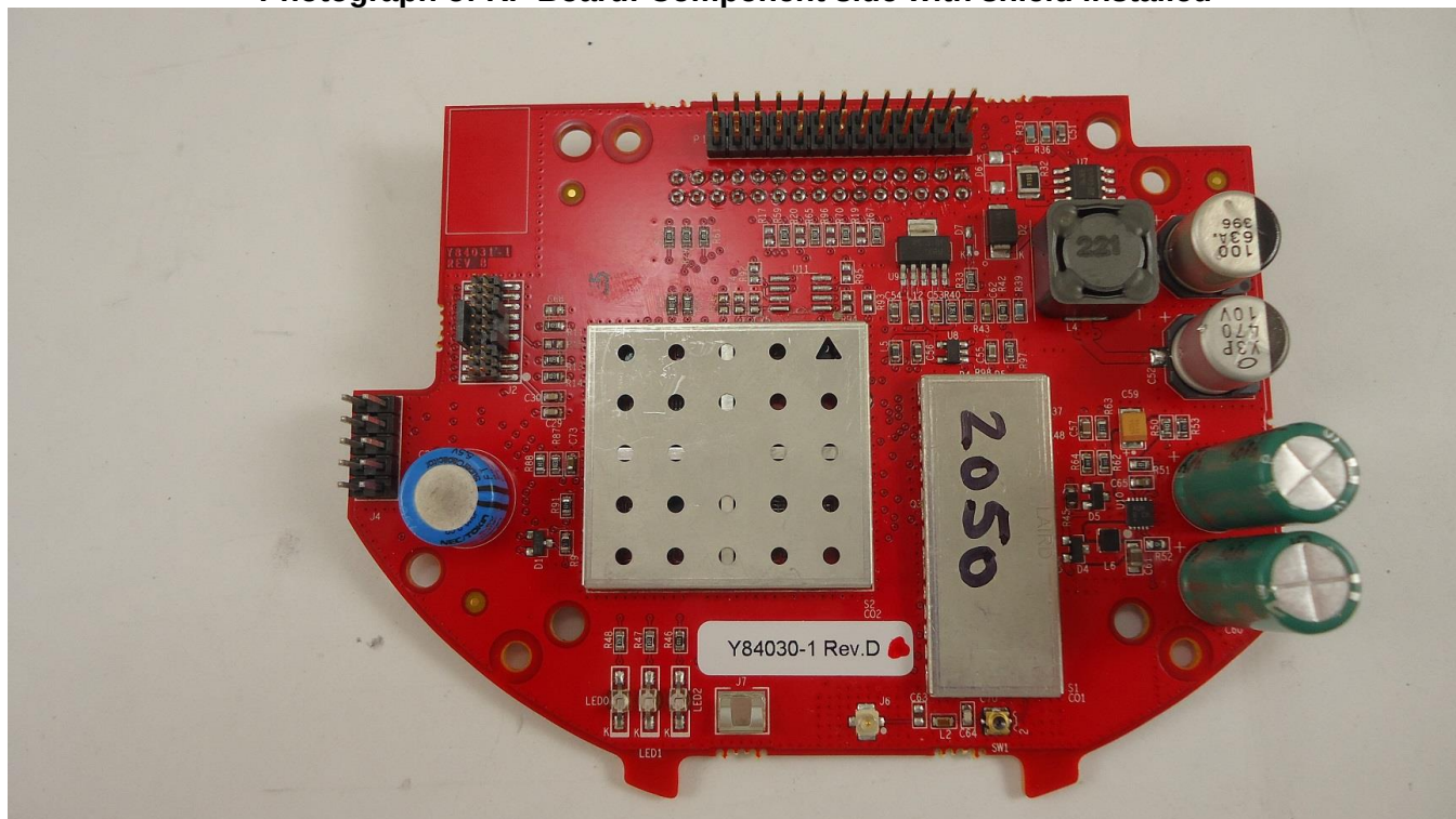
Photograph of RF Board: Component side with shield installed
