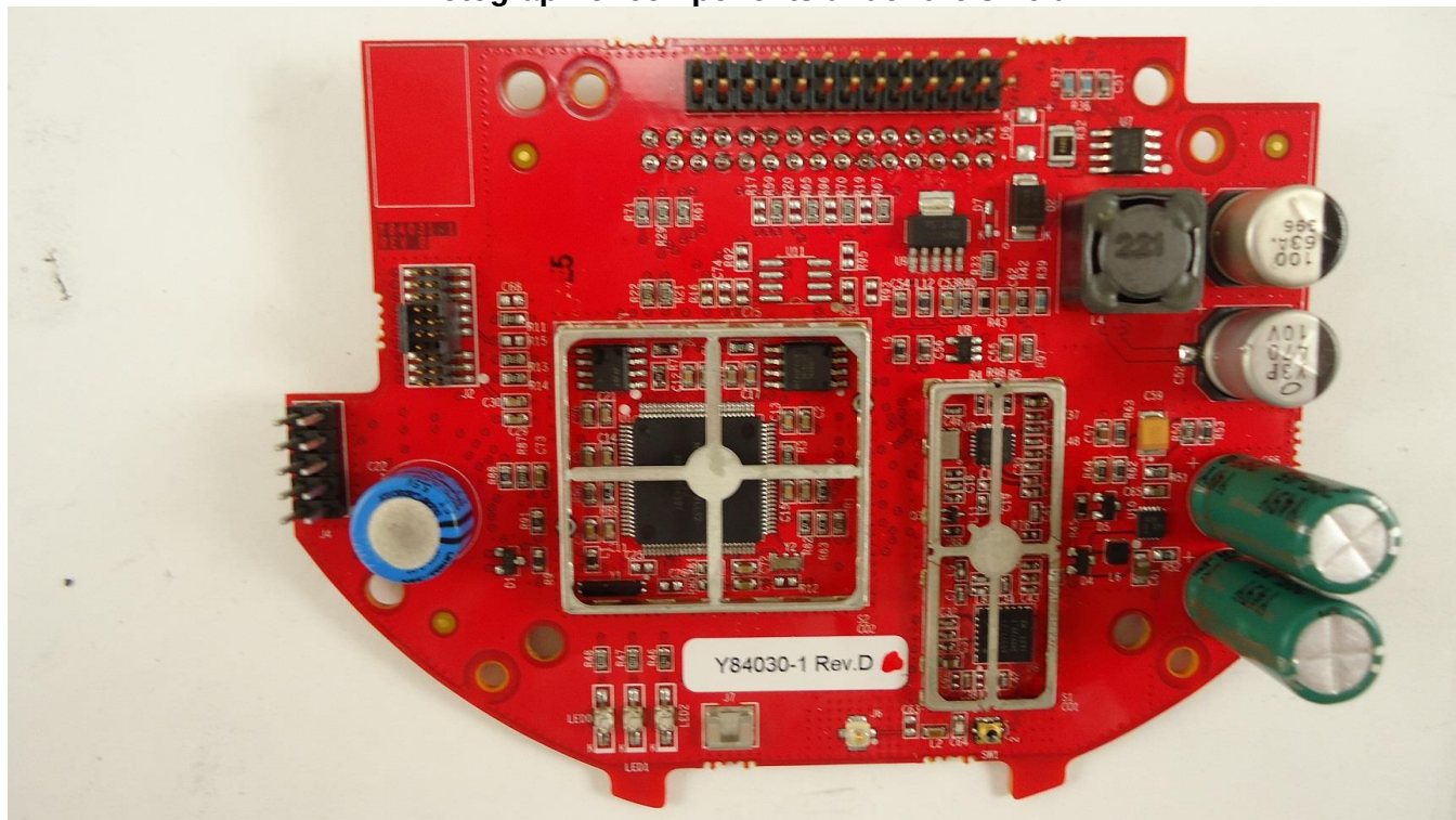
Photograph of components under the shield
