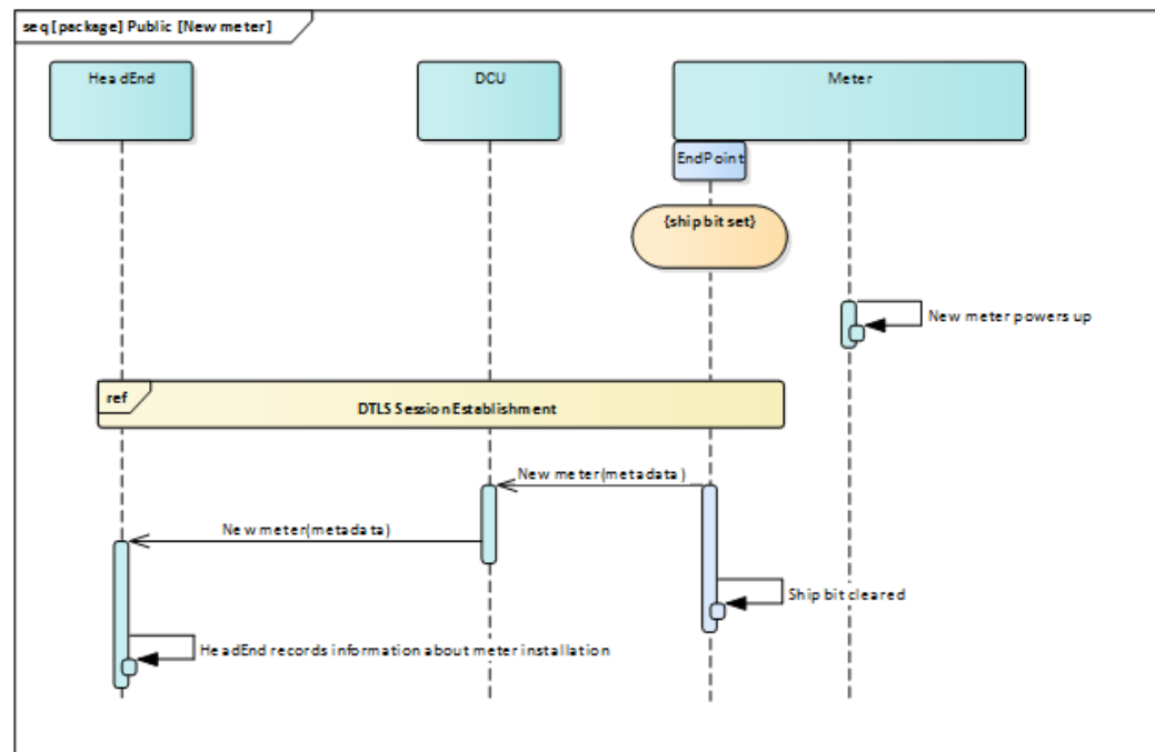
Figure 5.4 Meter Installation and Registration (SysML Sequence Diagram)
