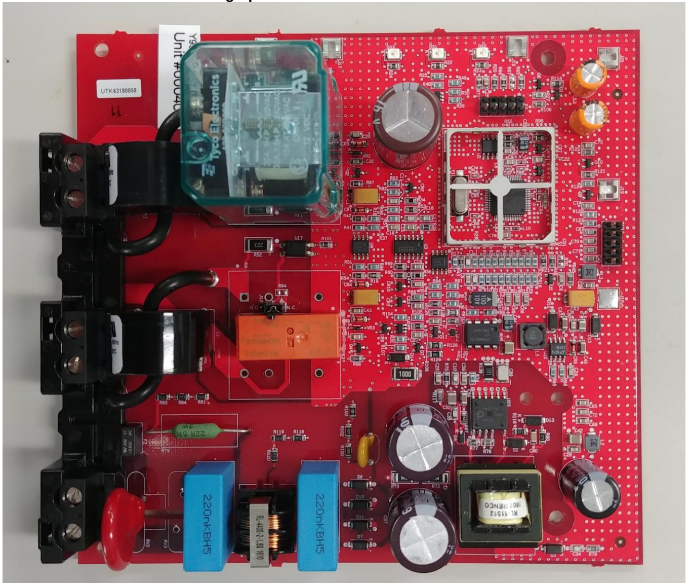
Photograph of Mother Board: Shield removed
