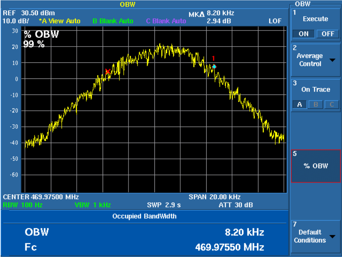
99% OBW 470 MHz
