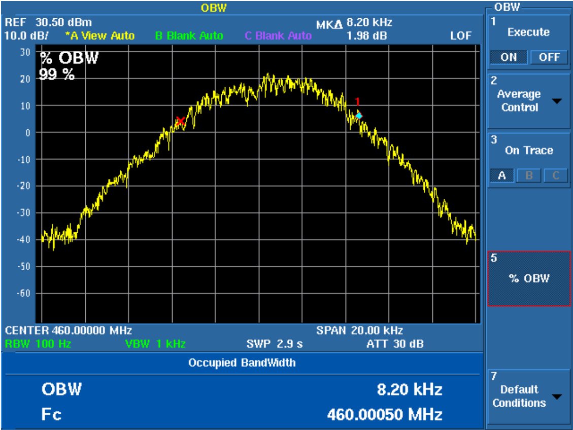
99% OBW 460 MHz
