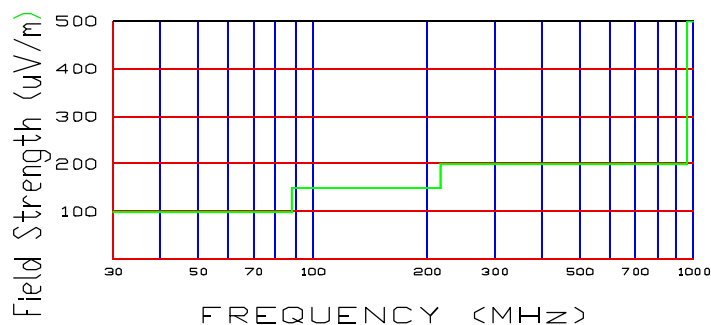
Fig. 10. Spurious Radiated Limits at 3 meters
