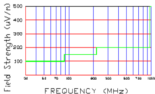
Figure 11. Spurious Radiated Limits at 3 meters
