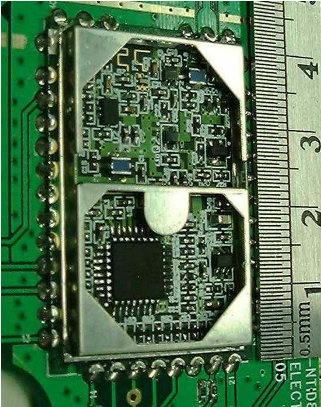
RF Module Circuit with RF Shield Removed
