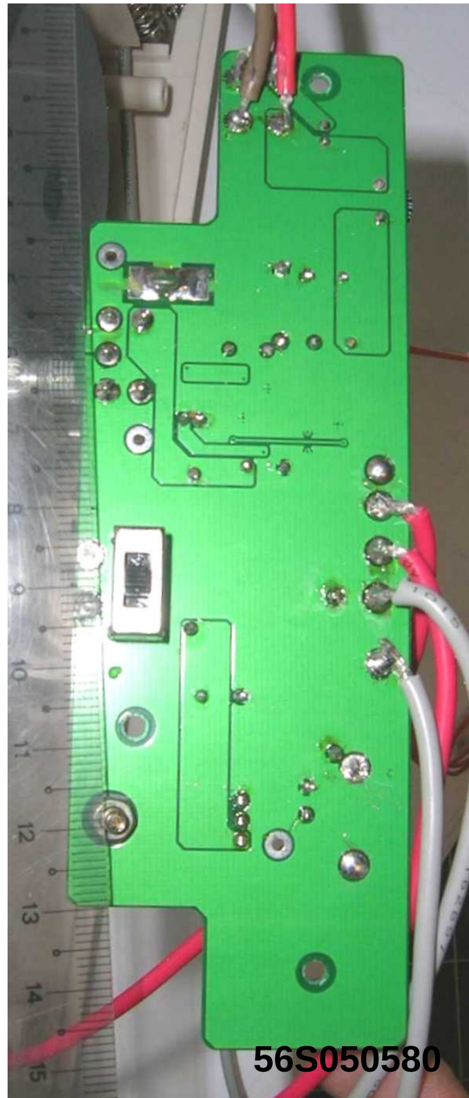
EUT PCB Sub-Board Trace Side
