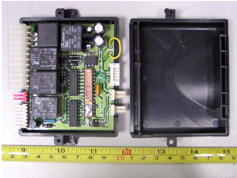
EUT –Base Uncovered view
