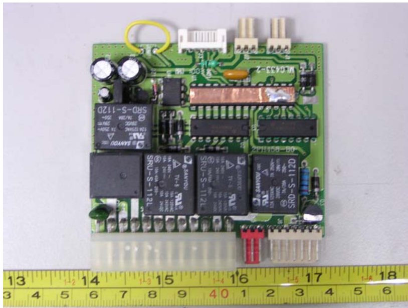
EUT –Base PCB front view
