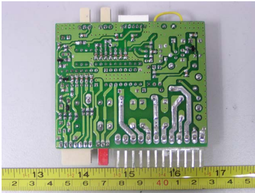
EUT -Base PCB back view
