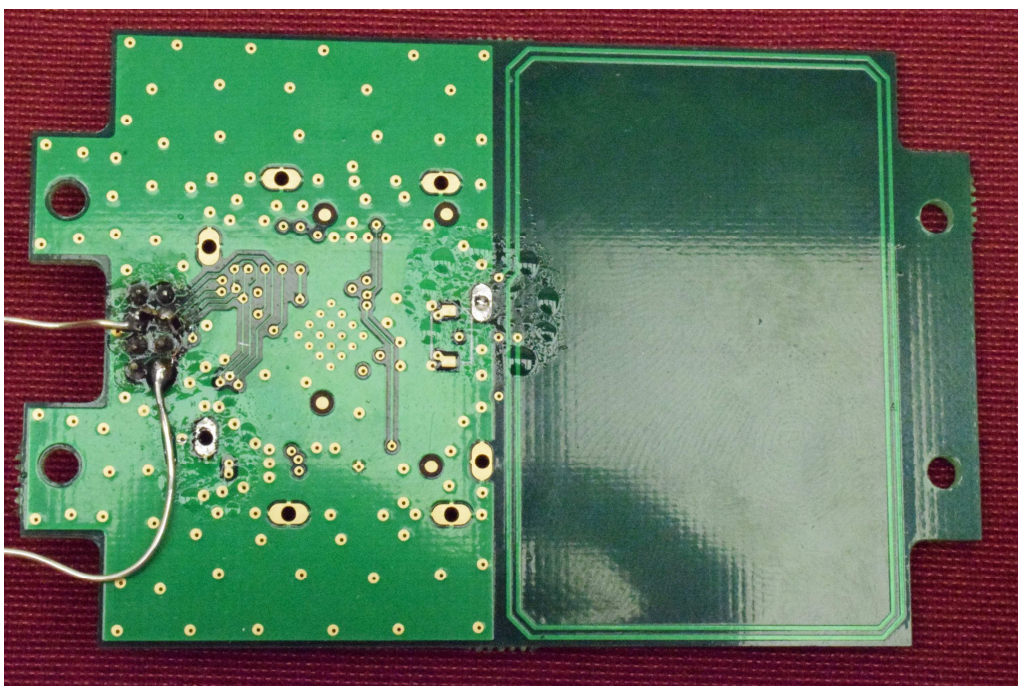
Picture 4: EUT without shielding (rear view)
