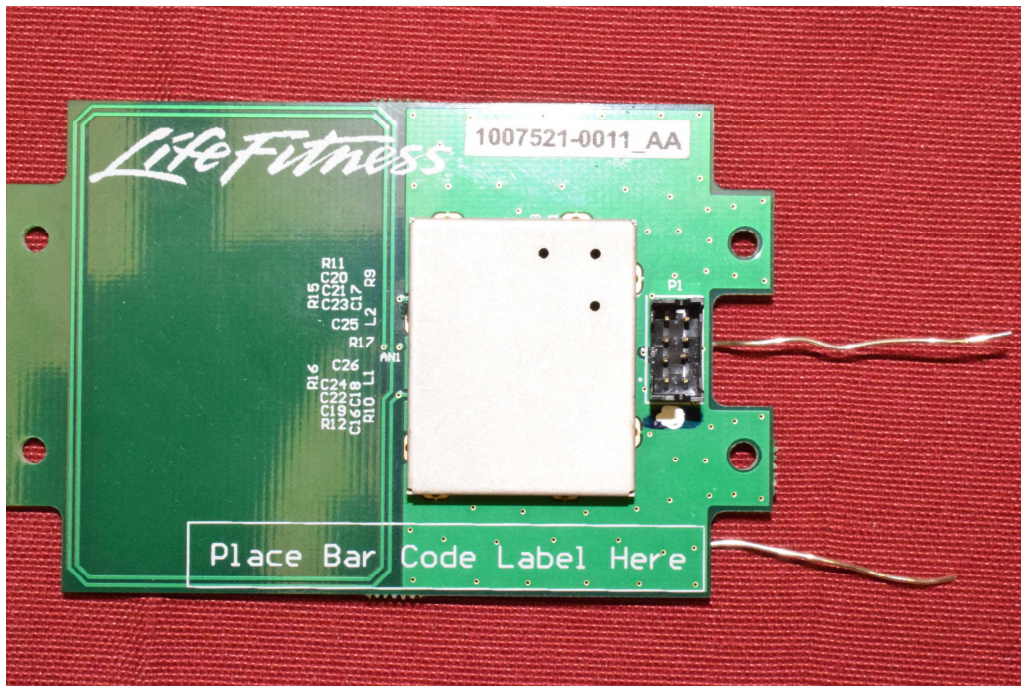
Picture 1: EUT (front view )
