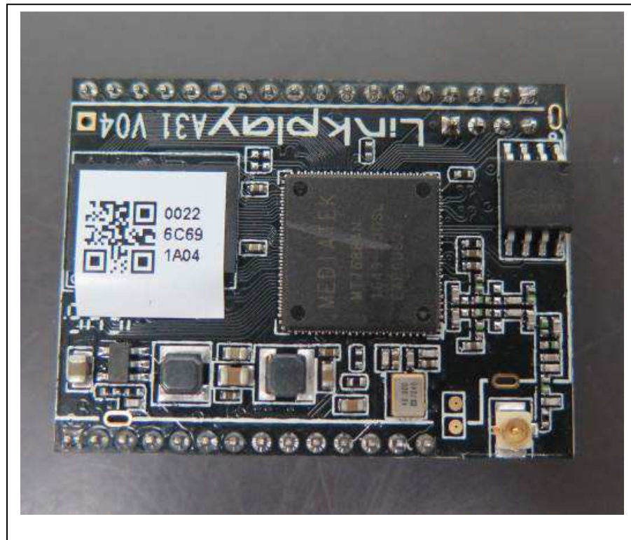
Internal Configuration 3 (Wi-Fi PCB)
