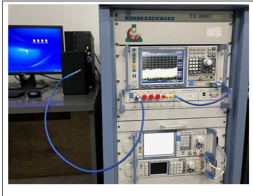
Test setup 1 (Wi-Fi and Bluetooth)
