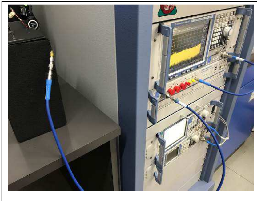
Test setup 2 (Wi-Fi and Bluetooth)
