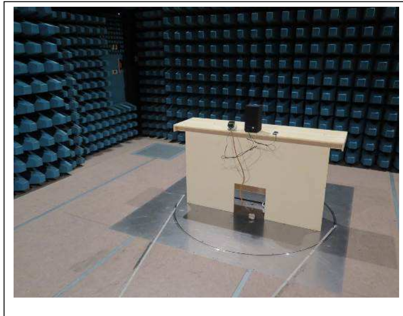
Test setup 5 for Aux in
