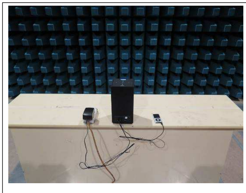
Test setup 6 for Aux in
