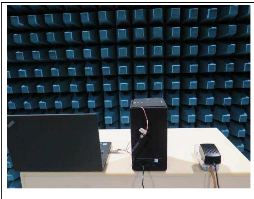
Test setup4 for Bluetooth and Wi-Fi
