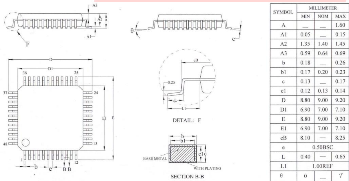
Figure 3-1. AC6921A_LQFP48 Package
