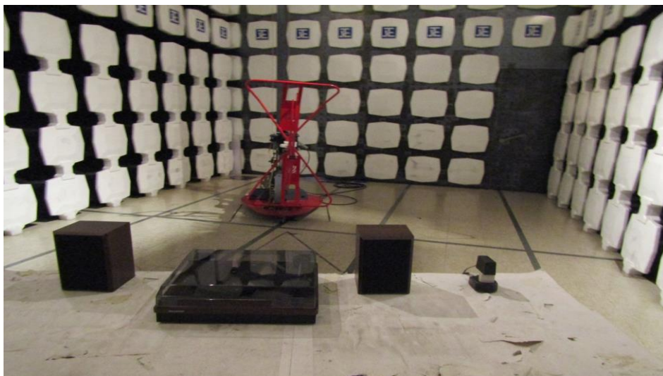
Measurement of Radiated Emission Test Set Up
