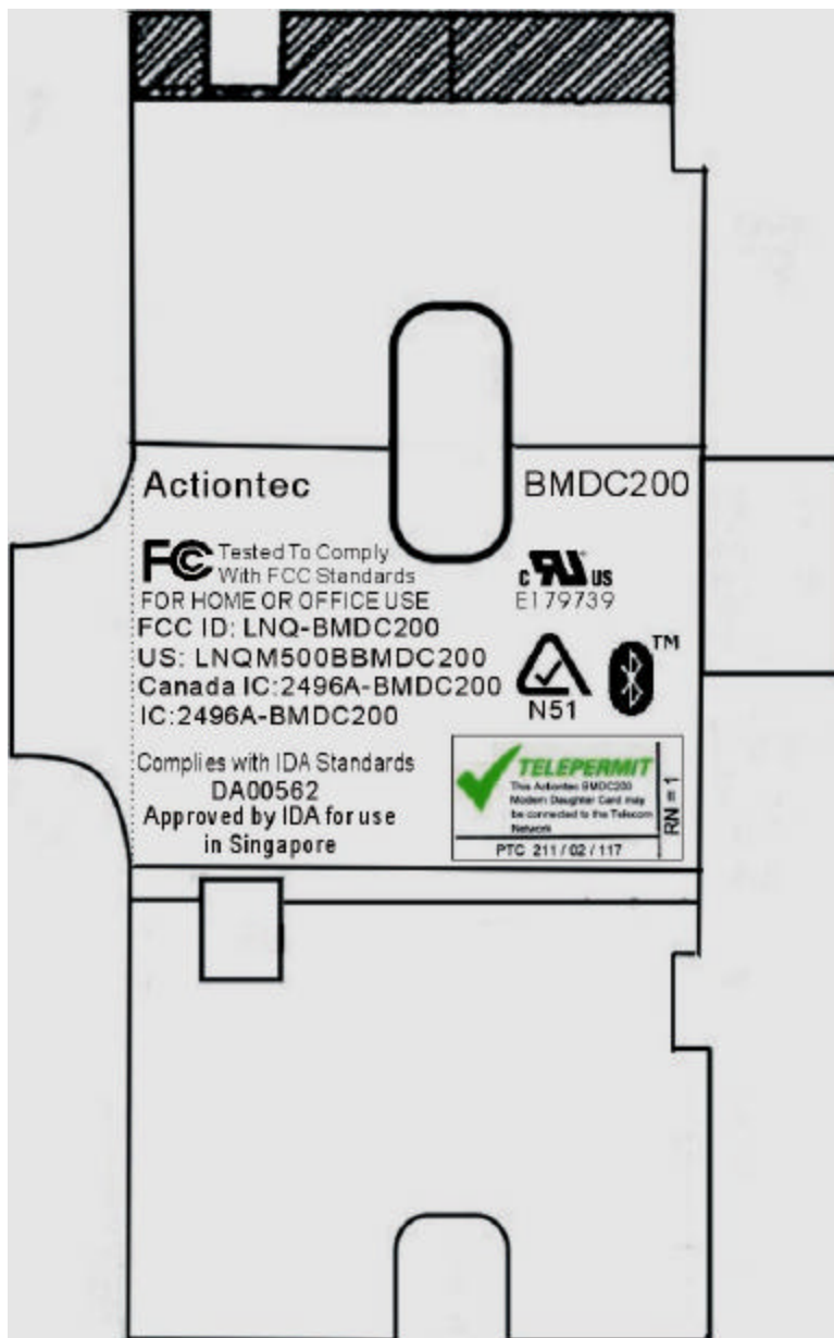
← Label drawing
