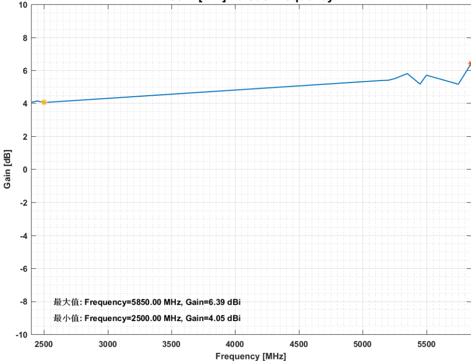
Gain [dBi] versus Frequency
