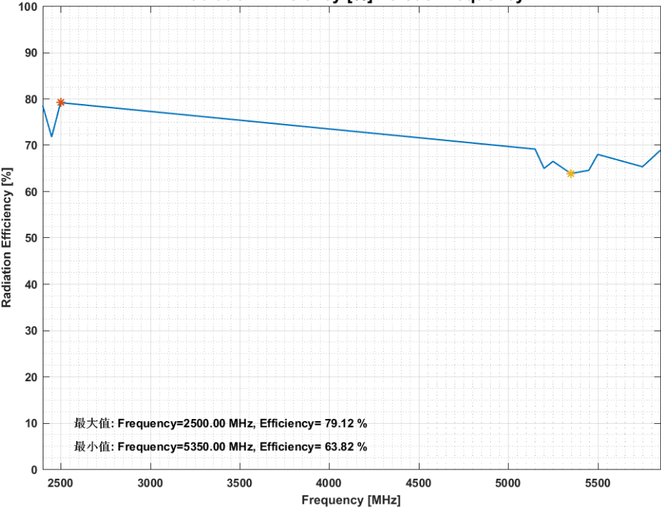
Radiation Efficiency [%] versus Frequency
