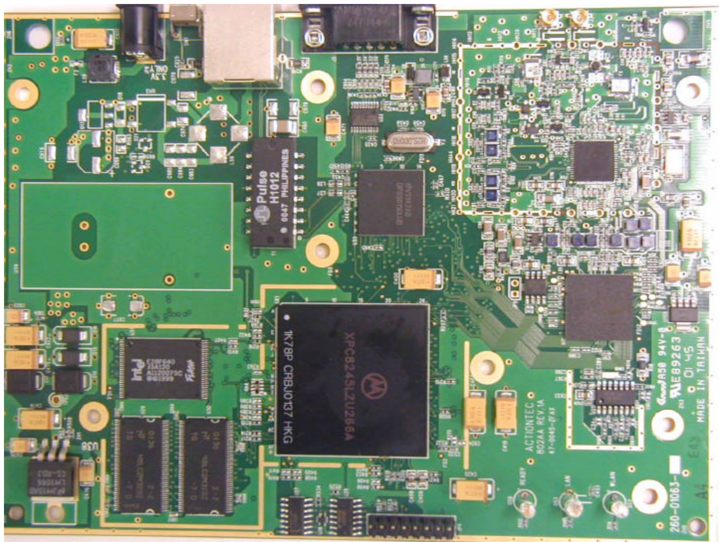
Top View of Board – Shield Removed
