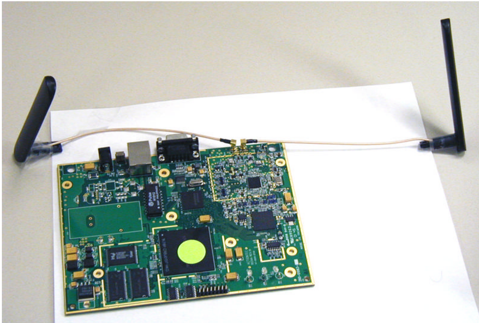
Assembly View showing how antennas are connected to the circuit board
