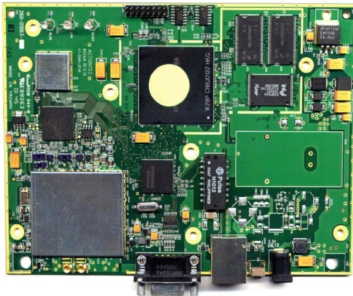
Top View of Board – Shield in Place
