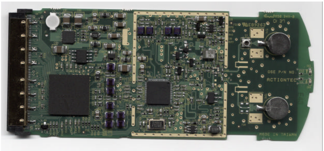
Top View of Board without shield
