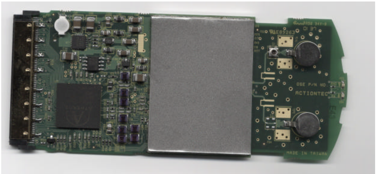
Top View of Board with shield
