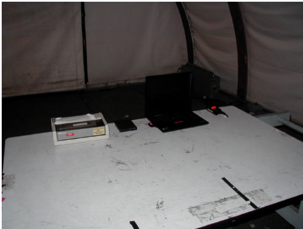
Radiated Emissions Below 1GHz (Radio Spurious Emissions and Digital Device)
