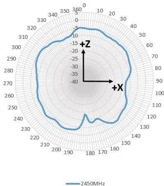
Elevation (XZ)
