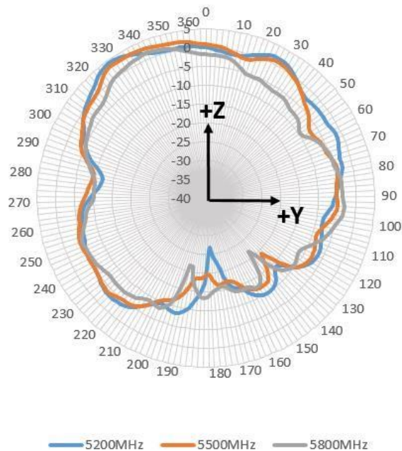
Elevation (YZ)
