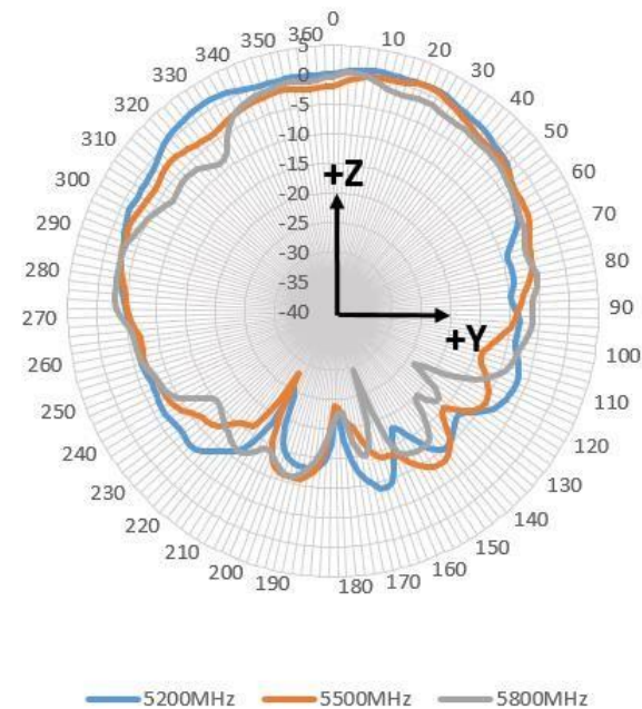
Elevation (YZ)
