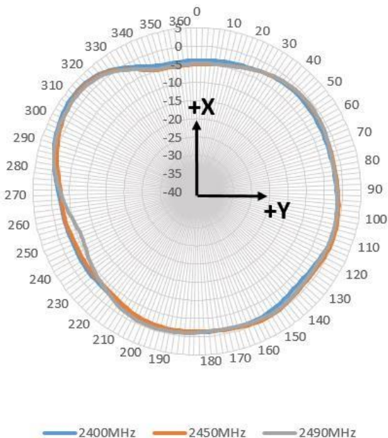
Azimuth (XY)
