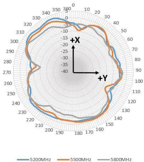
Azimuth (XY)
