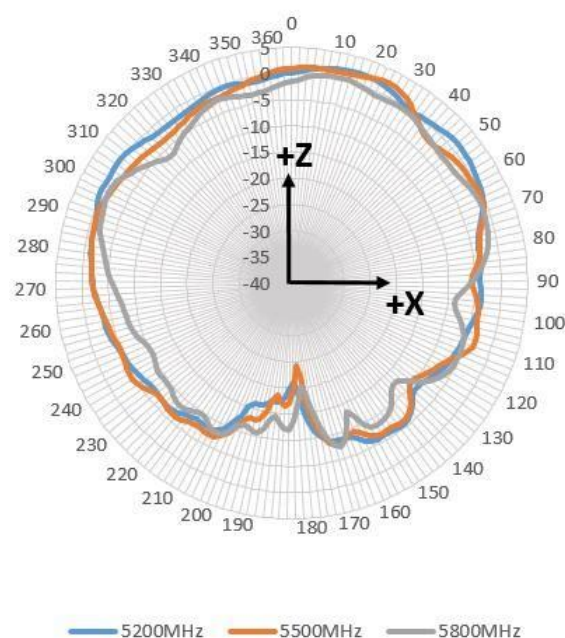
Elevation (XZ)
