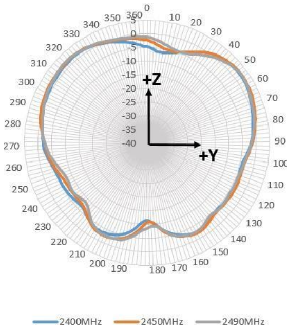
Elevation (YZ)
