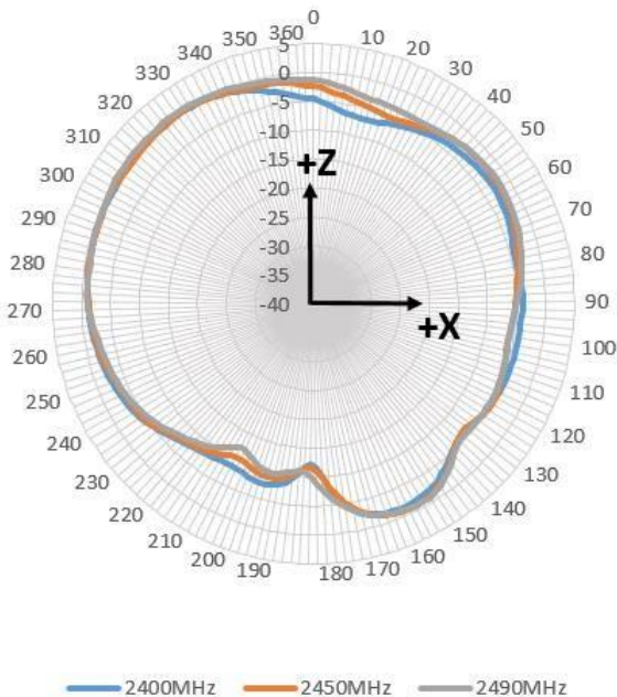
Elevation (XZ)
