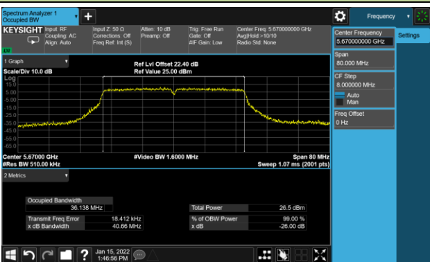
Channel 134 (5670MHz)
