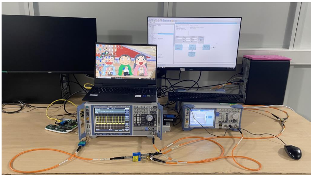
Description: DFS Test Setup
