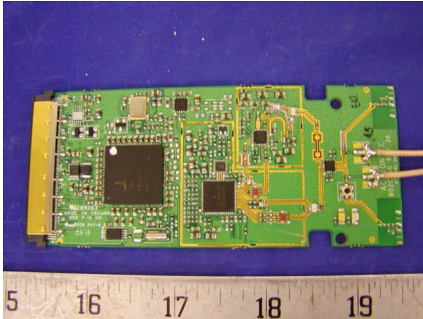
EUT – Transceiver Component View with Shield Removed
