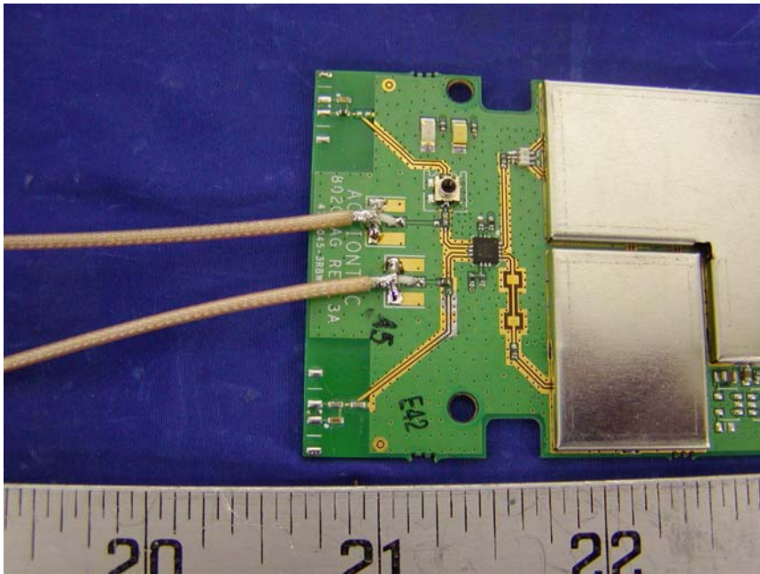
Antenna Connection View
