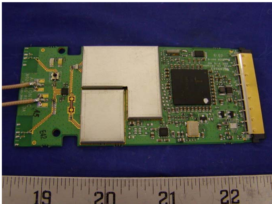
EUT – Transceiver Component View
