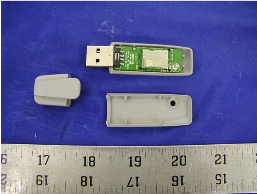
EUT – Cover Off Component View
