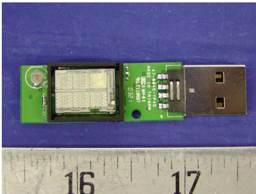
RF Module – Bottom With Antenna View
