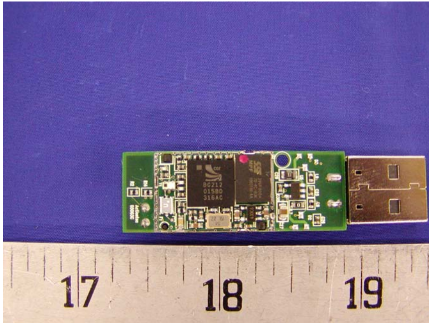
RF Module – Component View
