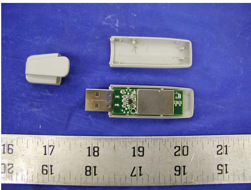
EUT – Cover Off Solder View
