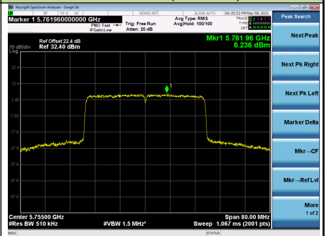
Channel 151 (5755MHz)
