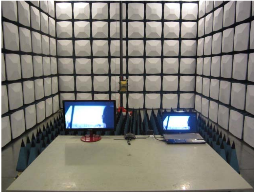
Radiated Emission – Front View (Above 1GHz Distance 3.0m)
