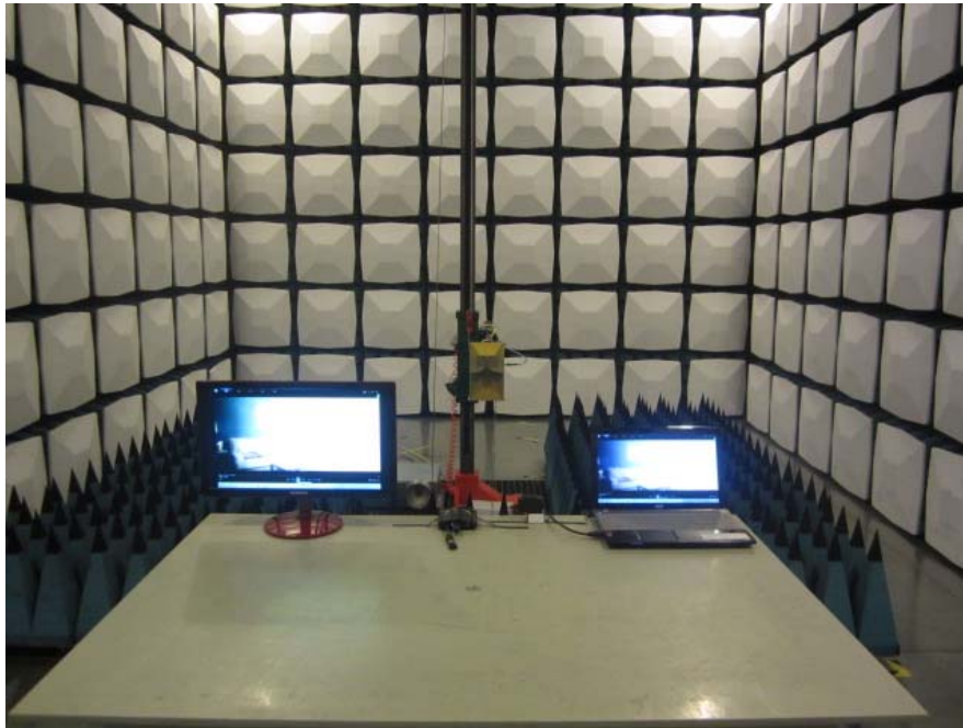
Radiated Emission – Front View (Above 1GHz Distance 1.5m)
