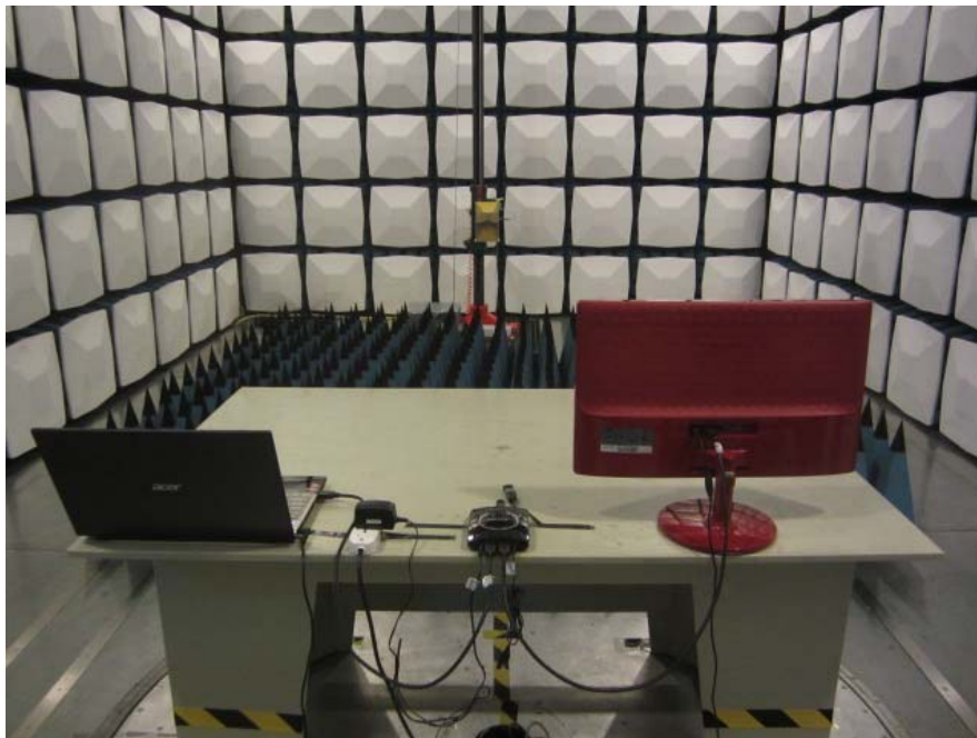
Radiated Emission – Rear View (Above 1GHz Distance 3.0m)
