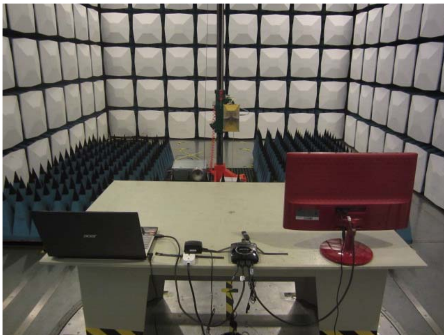
Radiated Emission – Rear View (Above 1GHz Distance 1.5m)
