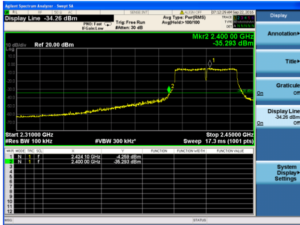
(802.11n-HT40) Band Edge-Low Channel
