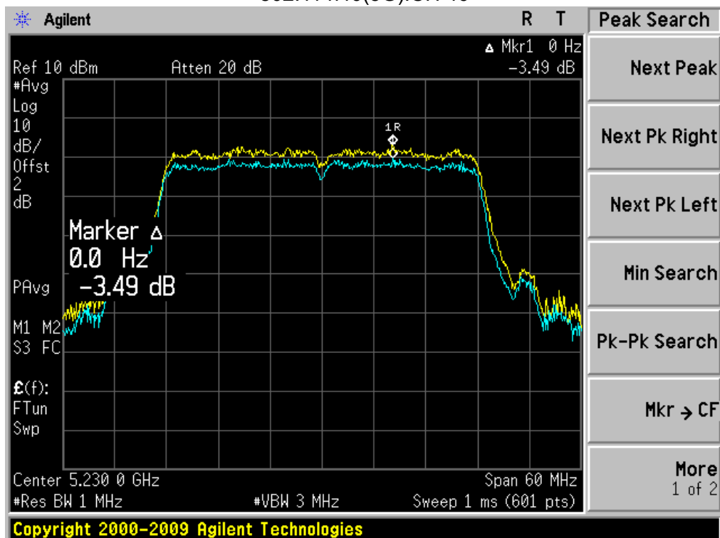
802.11 n40(5G):CH 46
