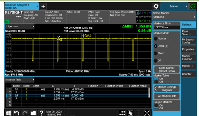
802.11ac-VHT20 (T = 1.311ms)
