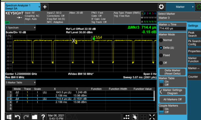
802.11ac-VHT40 (T = 646us)
