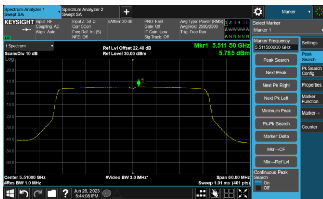
Channel 102 (5510MHz)
