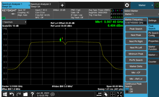
Channel 102 (5510MHz)
