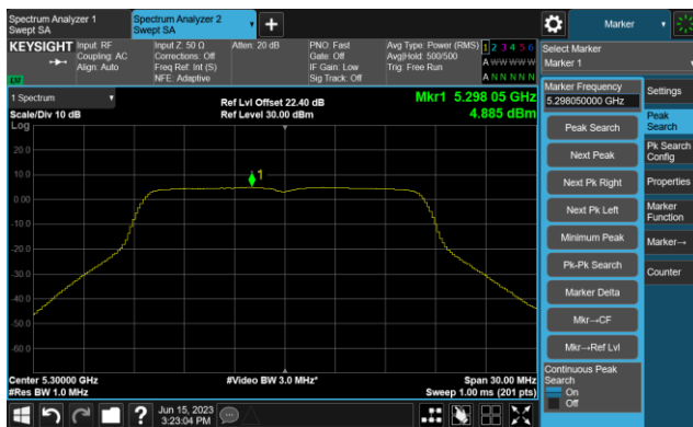
Channel 60 (5300MHz)
