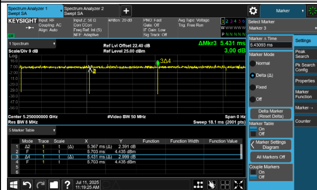
802.11ax-HE160 (T = 5.367 ms)
