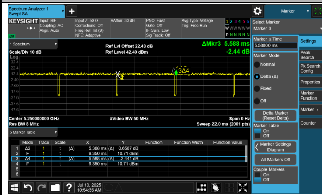
802.11ax-HE160 (T = 5.368 ms)
