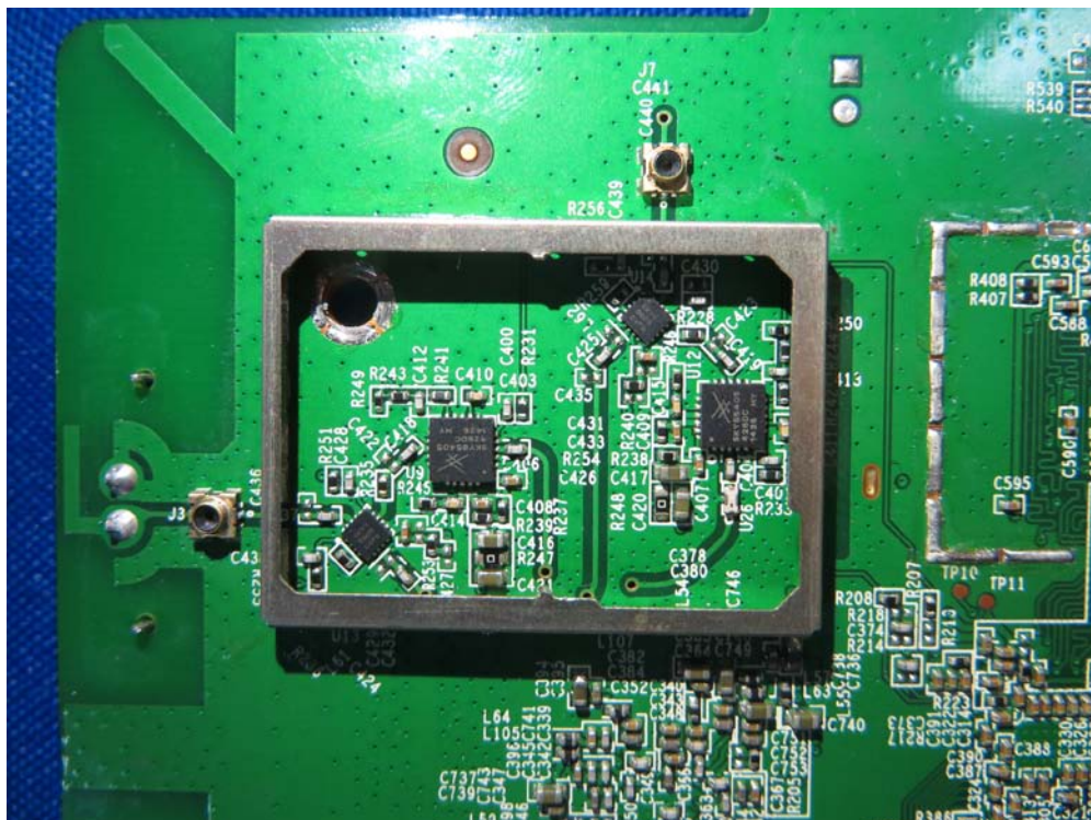
(34) EUT Photo (WEB6000Q)
