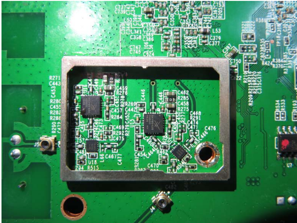
(26) EUT Photo (WCB6000Q)
