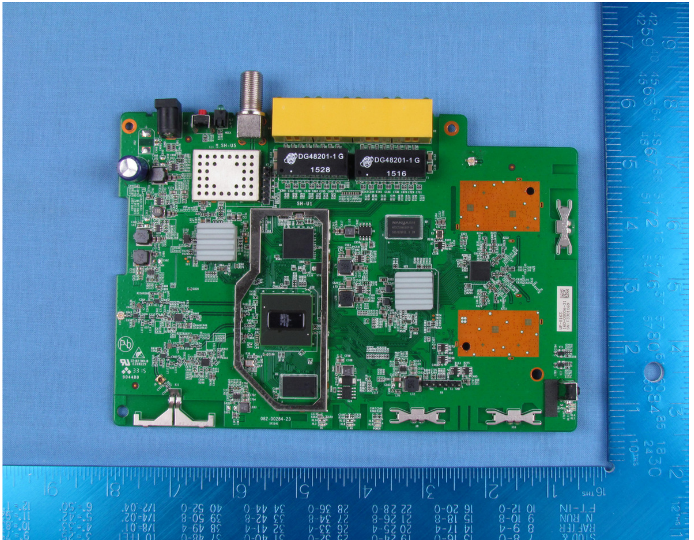
EUT – TOP VIEW
