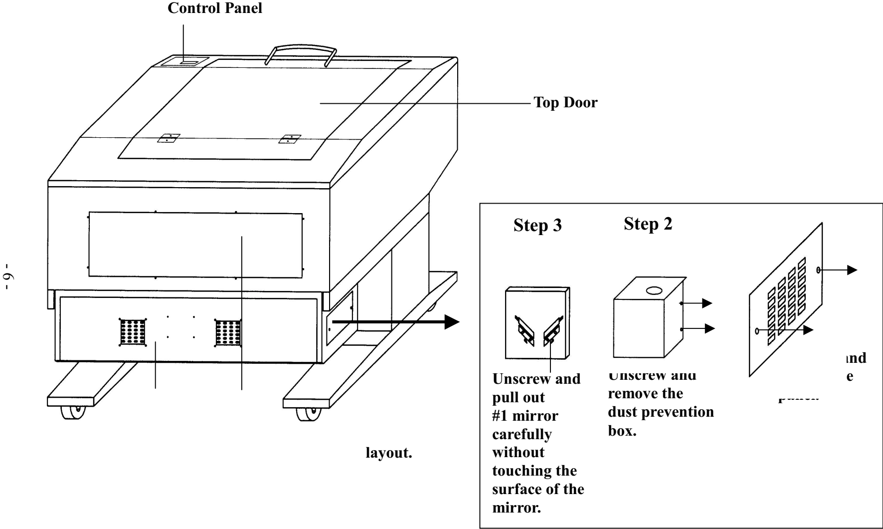
Fig. 2 Back View
