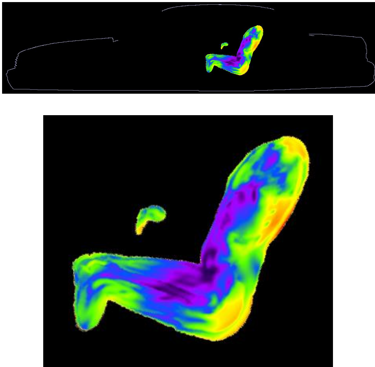
Figure 3. SAR distribution at 775.0000 MHz in the passenger model located on the side of the back seat, produced by the trunk-mount HAF4016A antenna. The contour plot is relative to the plane where the peak 1-g average SAR for this exposure condition occurs.
