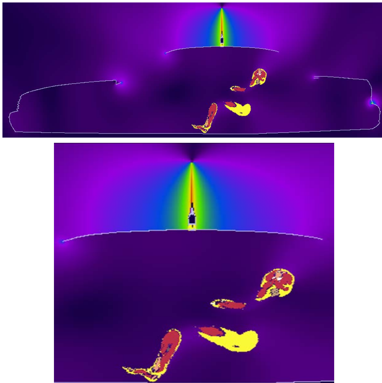
Figure 6. (a) E-field magnitude distribution corresponding to exposure condition of Figure 5, and (b) H-field magnitude distribution corresponding to exposure condition of Figure 5.
