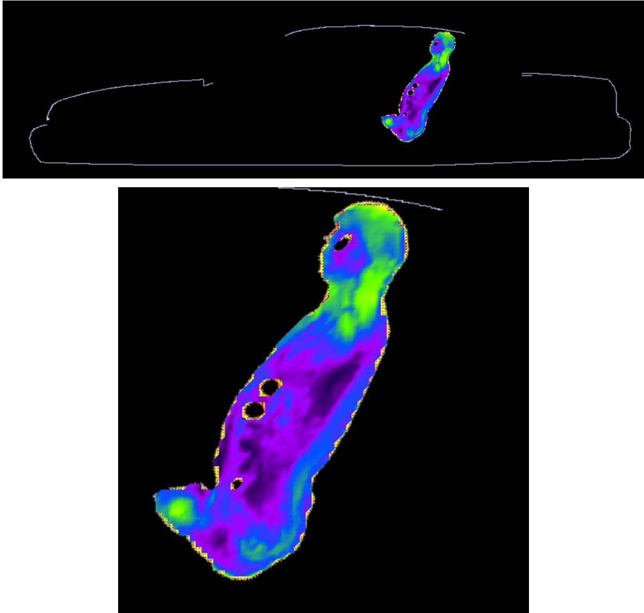
Figure 5. SAR distribution at 173.0125 MHz in the passenger model located on the side of the back seat, produced by the roof-mount AN000131A01 antenna. The contour plot is relative to the plane where the peak 1-g average SAR for this exposure condition occurs.
