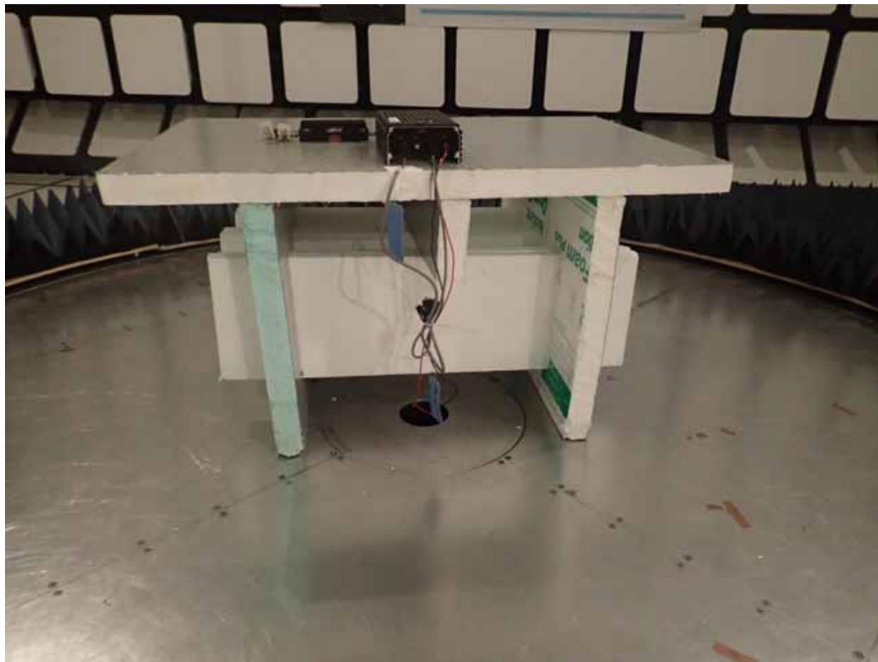
Radiated Emissions at 3 m
