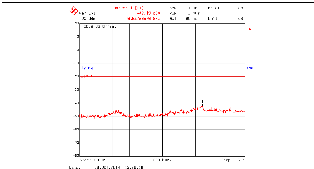
Plot 5.5.4.4. Conducted Transmitter Spurious Emissions, Low Power, 764.025 MHz, 1 GHz - 9 GHz
