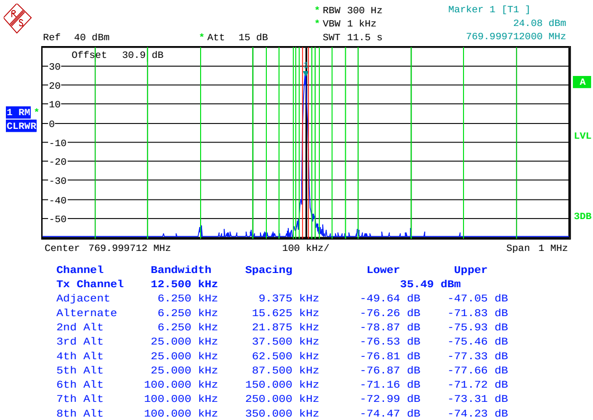
Plot 5.8.4.8. Adjacent Channel Power, Digital Mode, 12.5 kHz Channel Spacing, 770.0 MHz
