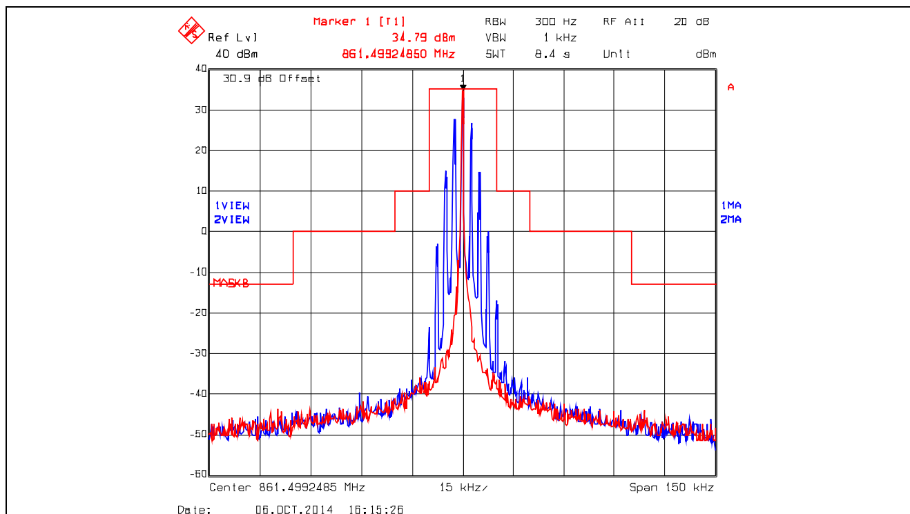
Plot 5.4.4.2.8. Emission Mask B, 12.5 kHz Channel Spacing, F3E, Low Power, 861.5 MHz
