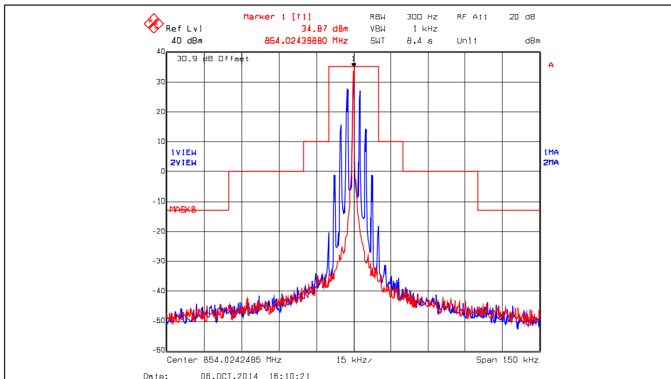
Plot 5.4.4.2.6. Emission Mask B, 12.5 kHz Channel Spacing, F3E, Low Power, 854.025 MHz
