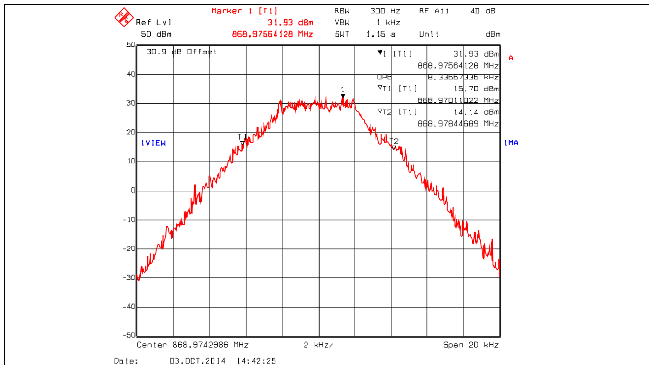
Plot 5.4.4.1.24. 99% Occupied Bandwidth, 12.5 kHz Channel Spacing, F1E/F1D, 868.975 MHz
