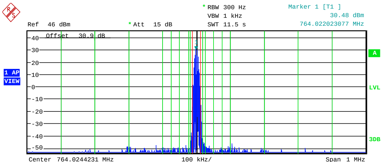
Plot 5.8.4.4. Adjacent Channel Power, Analog Voice, 25 kHz Channel Spacing, 764.025 MHz
