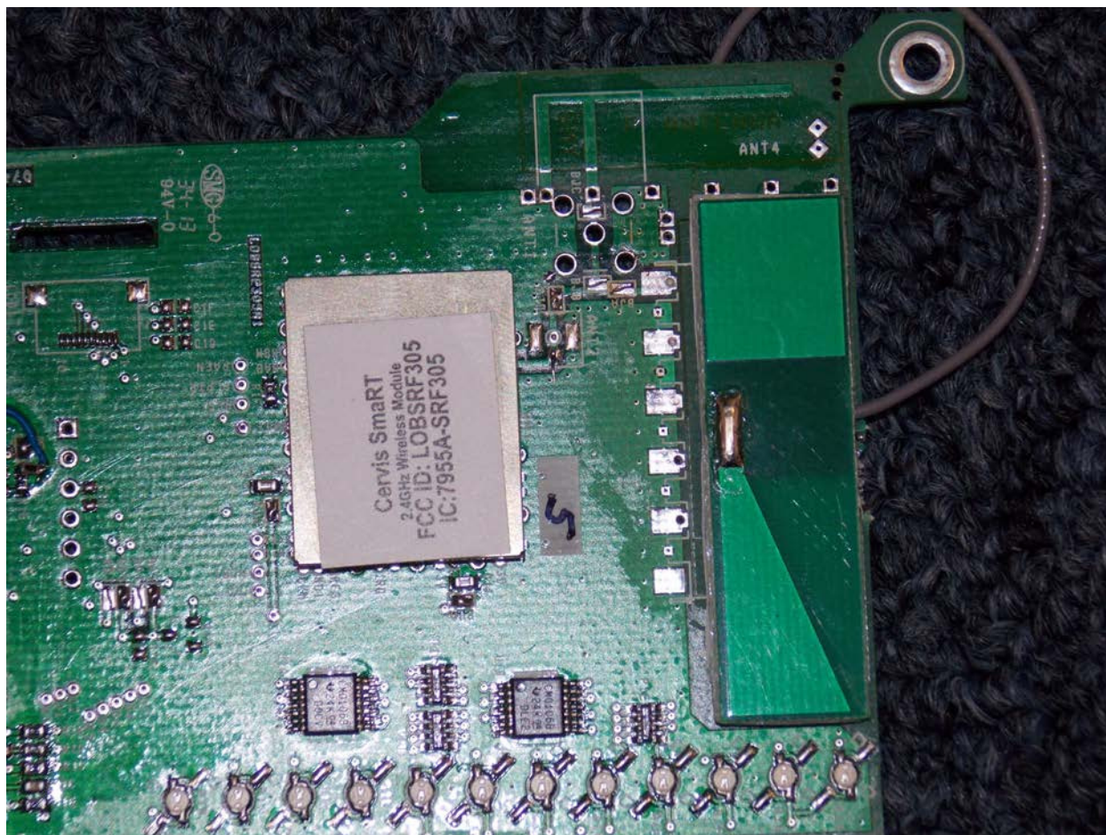
Module and Internal Antenna
