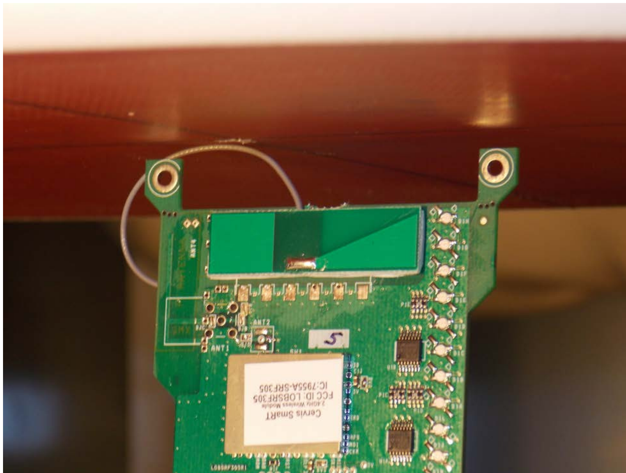
Test Position Internal Antenna Side F 3 mm Gap
