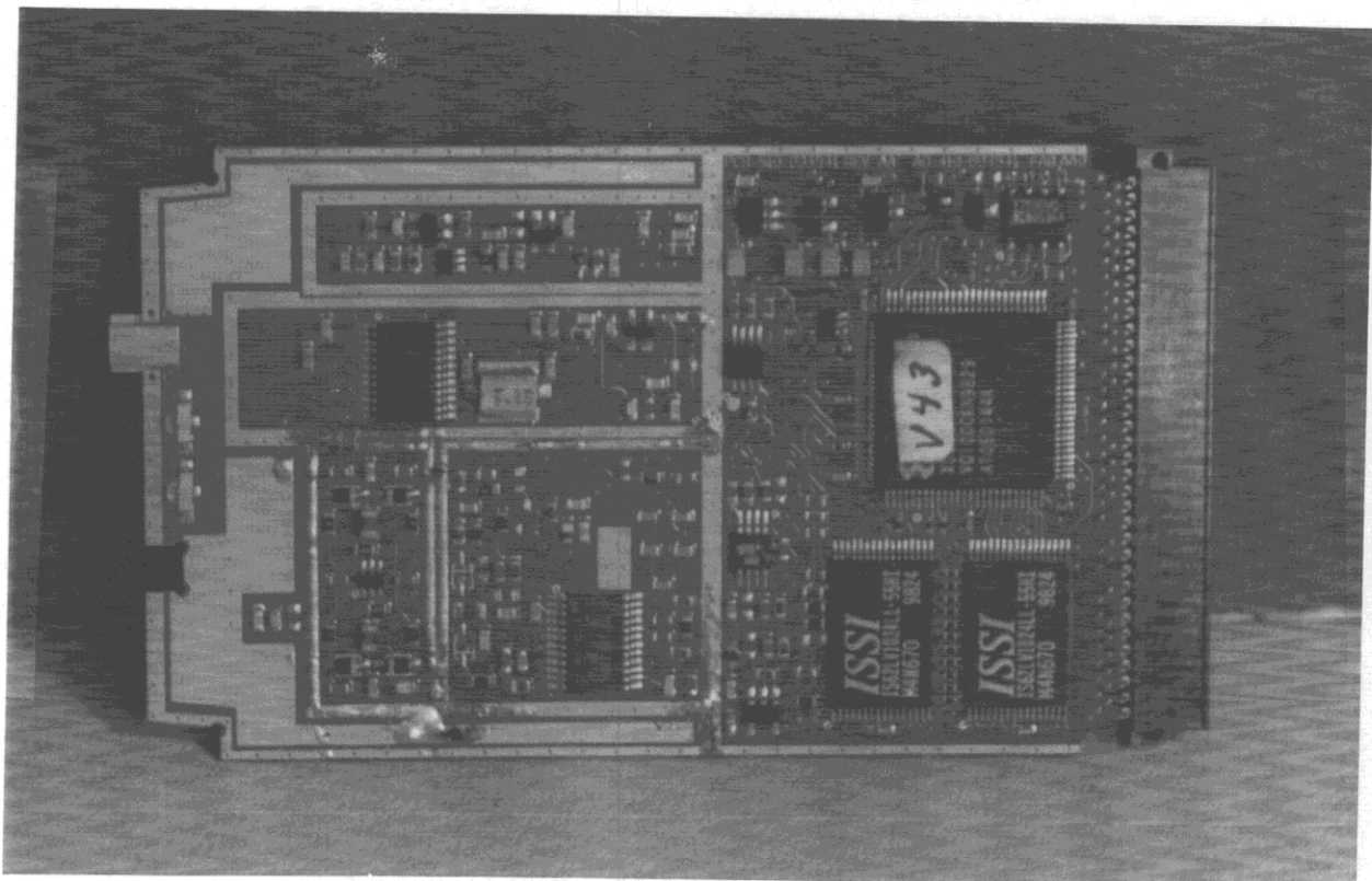
LM3100 PRINTED CIRCUIT BOARD - BOTTOM VIEW
