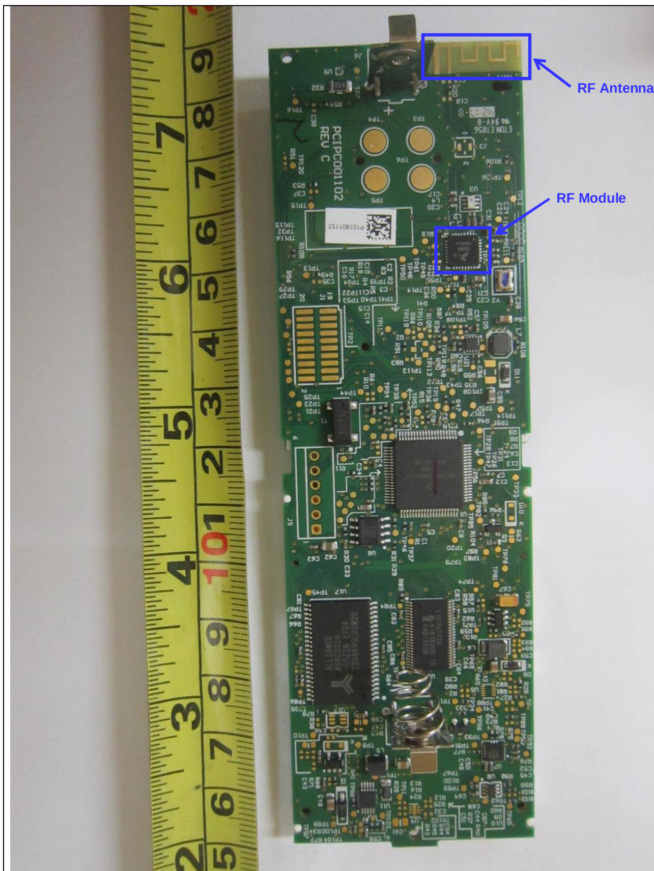
7RF Module Circuit with RF Shield Removed
