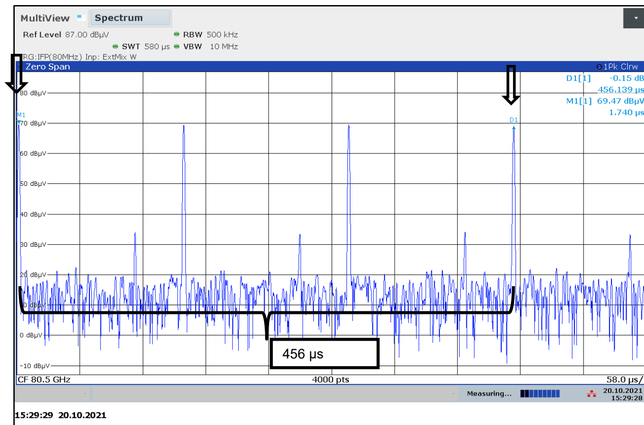
Plot 4-1: 456 microsecond Signal Sweep
