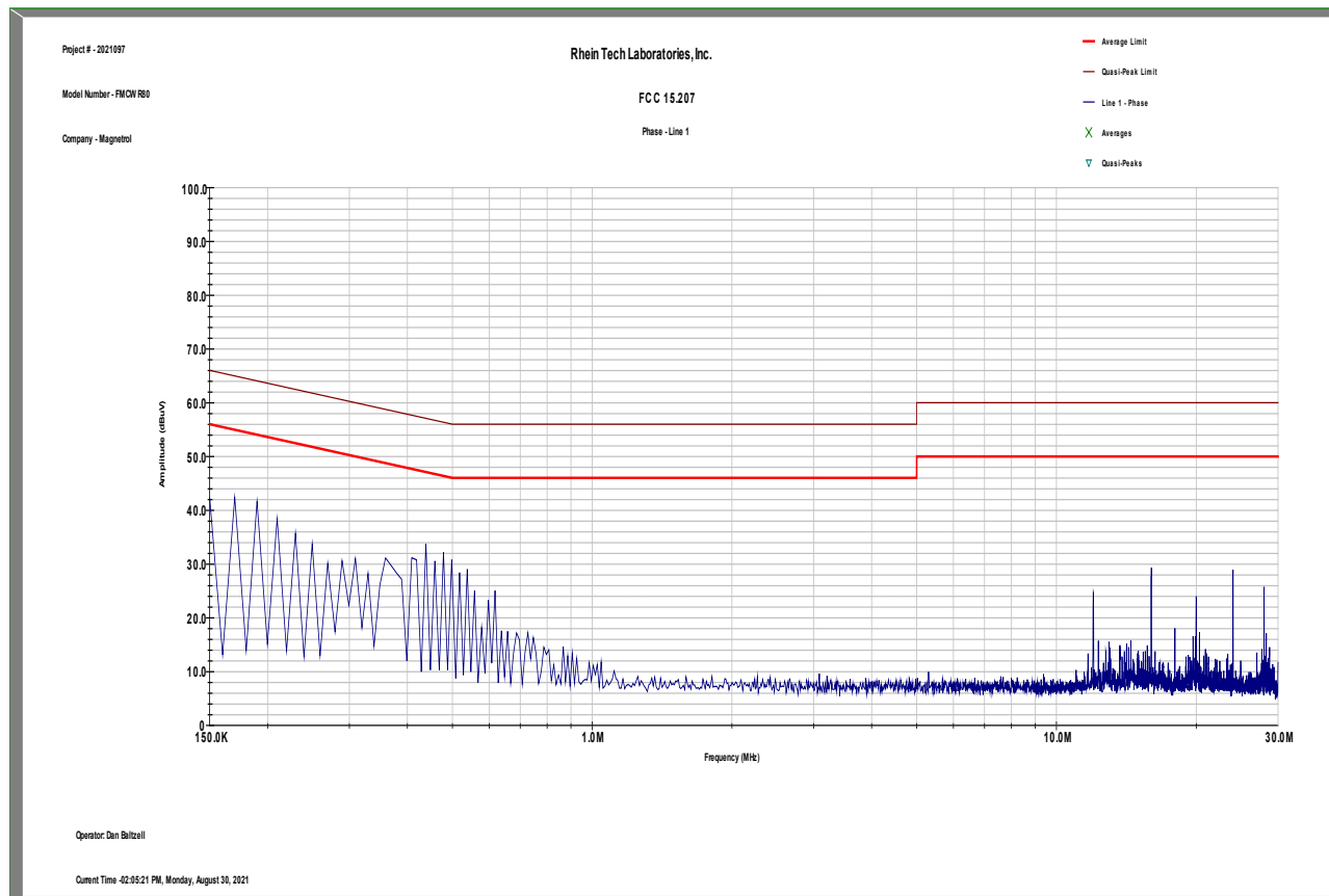
Plot 3-1: Conducted Emissions Transmit - Phase
