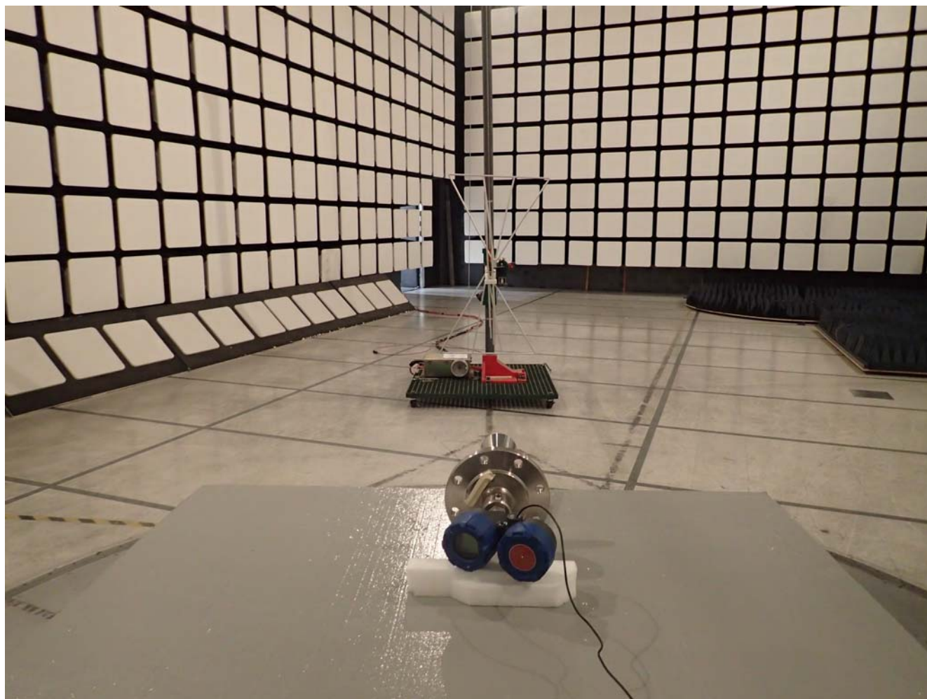
LPR Radiated Emissions at 3 m Distance (30 - 1000 MHz)
